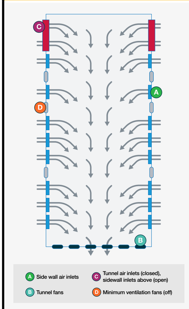
Figure 106 Typical air movement during transitional ventilation.
